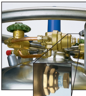
MCR models have a combination pressure control regulator with an exclusive, calibrated micrometer adjusting screw. (MP & HP models only)
